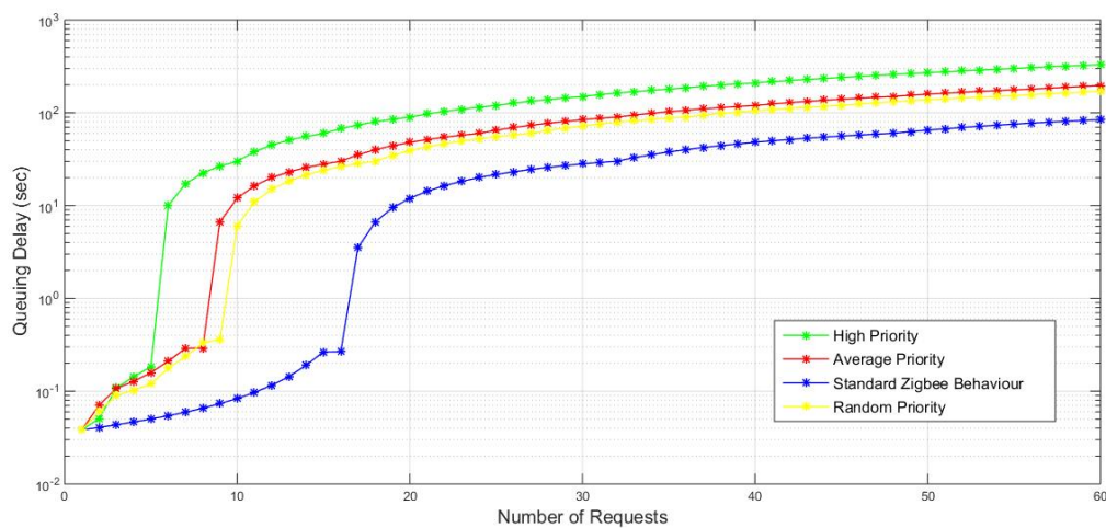
Fig 4: Delay Graph for Zigbee
